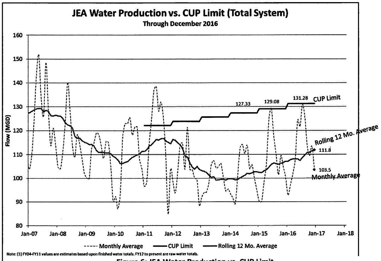
Figure 6: JEA Water Production vs. CUP Limit
